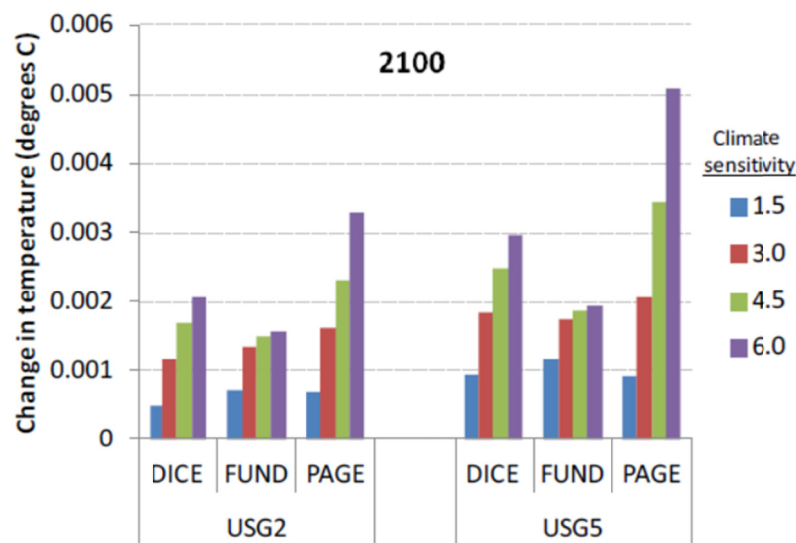
FIGURE 4-3 Projected incremental global mean temperature increase in 2100 of the SCC-IAMs.
