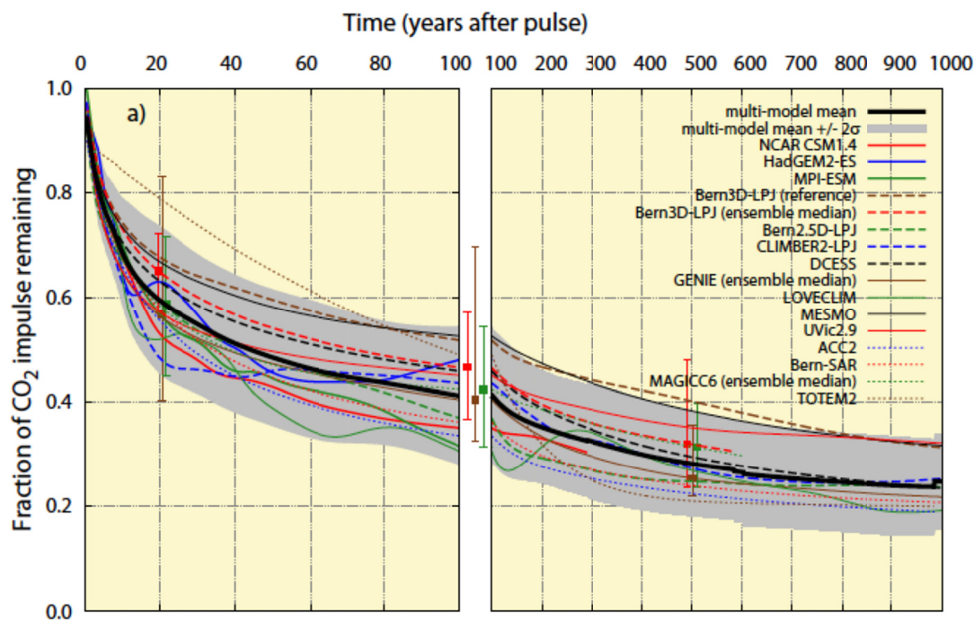
FIGURE 3-4 The perturbation to atmospheric CO 2 concentrations in response an emission pulse.
